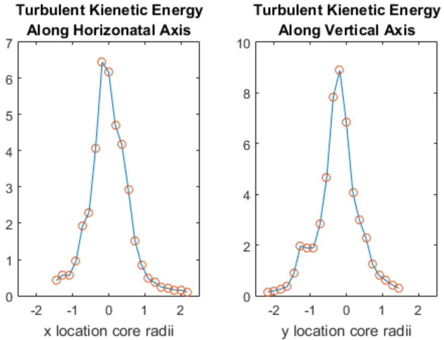
Figure 58 Turbulent Kienetic Energy 10.5 Chord Lengths downstream of the vortex generator at a tunnel velocity of 40 m/s.
