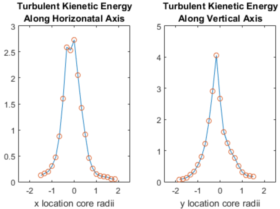
Figure 56 Turbulent Kinetic Energy 10.5 Chord Lengths downstream of the vortex generator at a tunnel velocity of 30 m/s.
