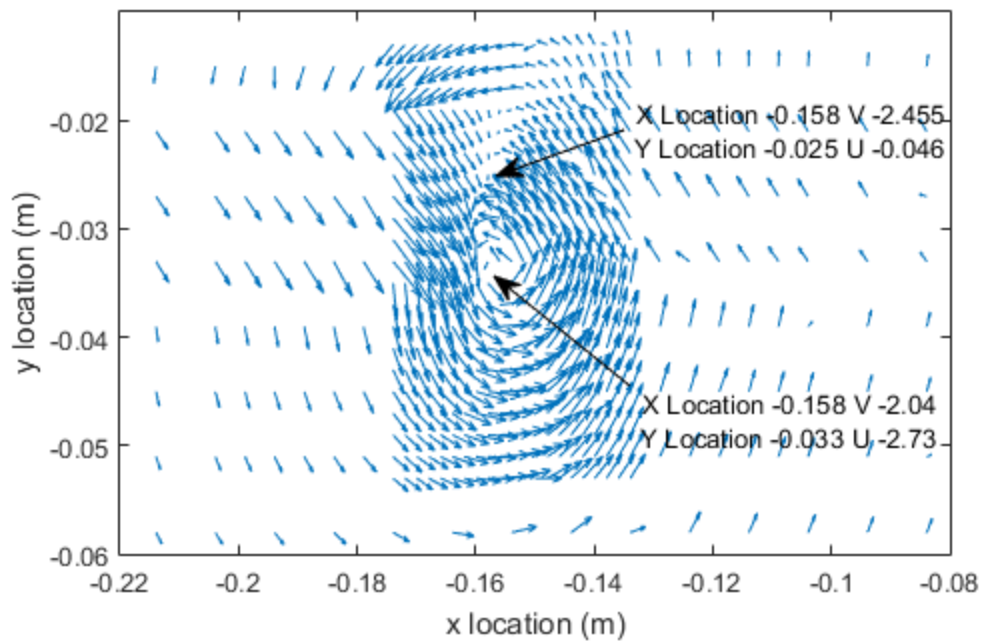
Figure 34 Mean velocity vector field seven chord lengths behind bi-wing generator, free stream velocity of 40 m/s displaying partially-merged co-rotating vortices
