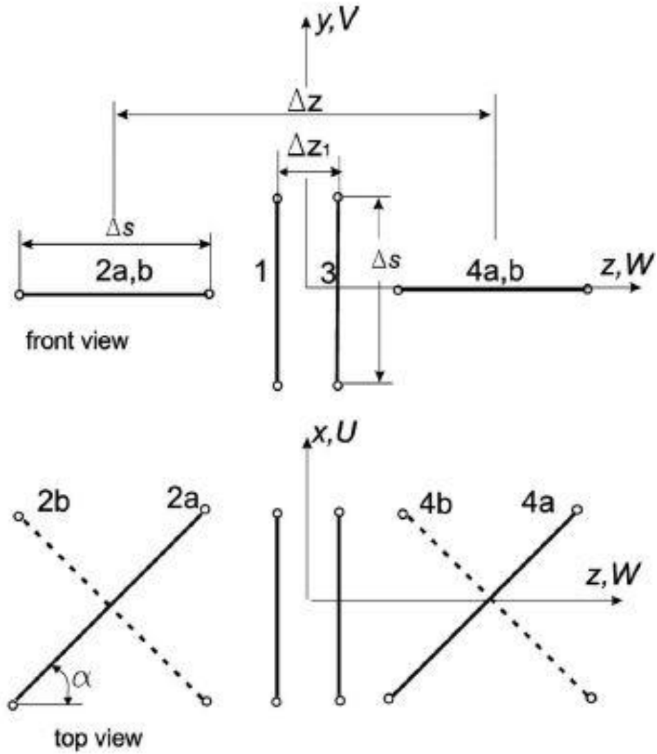
Figure 1 XP probe configuration (Vukoslavcevic and Wallace 2013)
